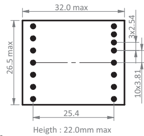
EF 25 reinforced insulation creepage distances: 8mm
