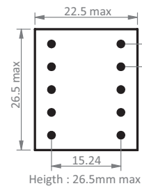
E 25 reinforced insulation creepage distances: 8mm
